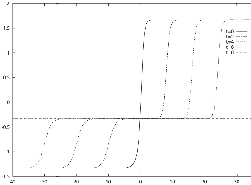
Fig. 5.4 KPP, collision of two fronts. The function u(x, t) is plotted as a function of x at the successive times t = 0, 2, 4, 6, 8 , with the parameters values b = 1, d = 1, e_j = (0, 2, -1), C_j = (1, 1, 1) .
